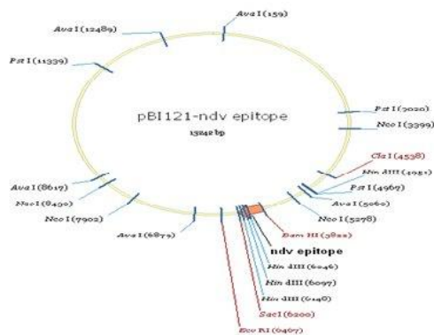
Figure 2. Schematic structure of the recombinant plasmid pBI121- NDV epitope for Agrobacterium-mediated transformation of tobacco hairy root. The DNA sequence encoding NDV epitope was cloned the downstream of the CaMV 35S promoter of a binary plasmid pBI 121
